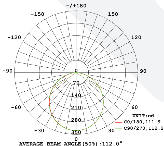
Light distribution
